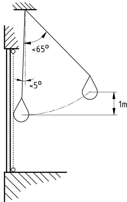
Figure 2 – Test apparatus for impact test
